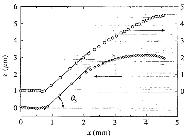
FIG. 2. Contour (viewed from the side) of the liquid surface vs distance x measured from the left end of the 4.7-mm-long lines marked in Figs. 1(b) (O) and 1(c) (◇); both dark and bright fringes were employed in the analysis. Least-squares-fitted straight lines in the region 0.8 \text{ mm} < x < 1.8 \text{ mm} yield for the inclination angle \theta_3 = 1.68 \text{ mrad} (O) and 1.78 \text{ mrad} (◇), respectively. Note the different vertical and horizontal scales.
